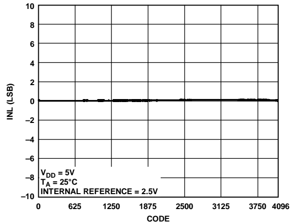
Figure 14. AD5694R INL
