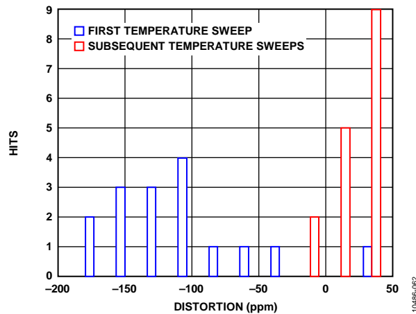
Figure 55. Thermal Hysteresis
