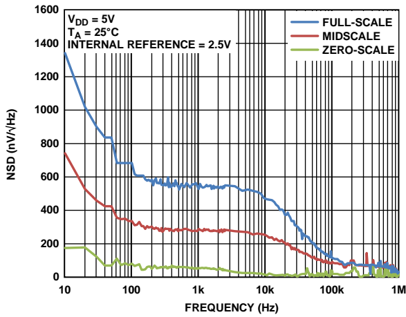
Figure 41. Noise Spectral Density
