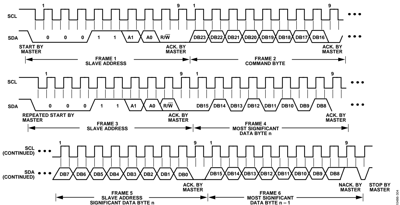
Figure 51. I 2 C Read Operation
