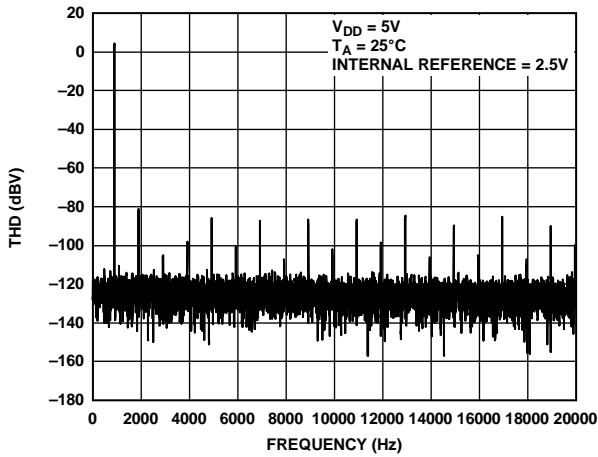
Figure 42. Total Harmonic Distortion at 1 kHz
