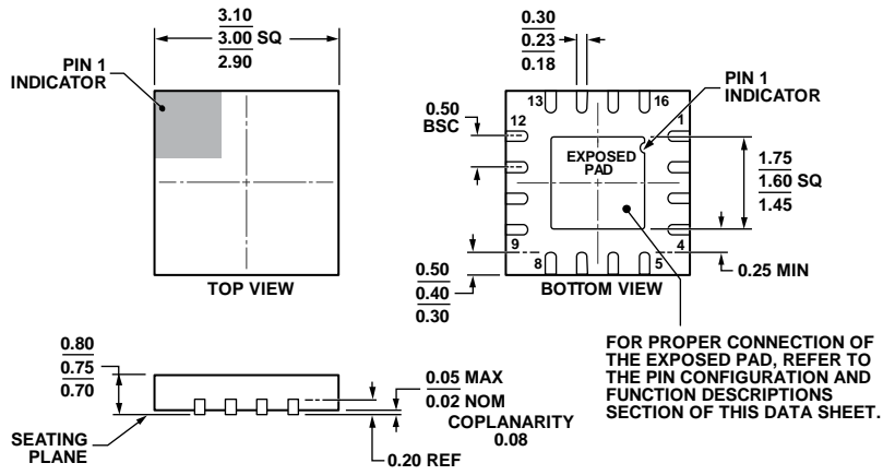
Figure 59. 16-Lead Lead Frame Chip Scale Package [LFCSP_WQ] 3 mm x 3 mm Body, Very Very Thin Quad (CP-16-22)
