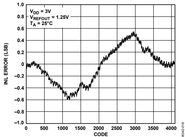
Figure 20. AD5627R INL, 1.25 V Internal Reference
