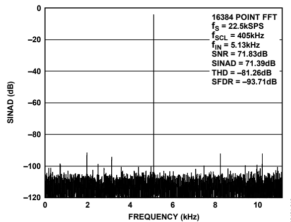
Figure 15. Dynamic Performance, f_{SCL} = 405kHz Without Clock Stretching, V_{DD} = 5V , Full-Scale Input, Seven-Term Blackman-Harris Window
