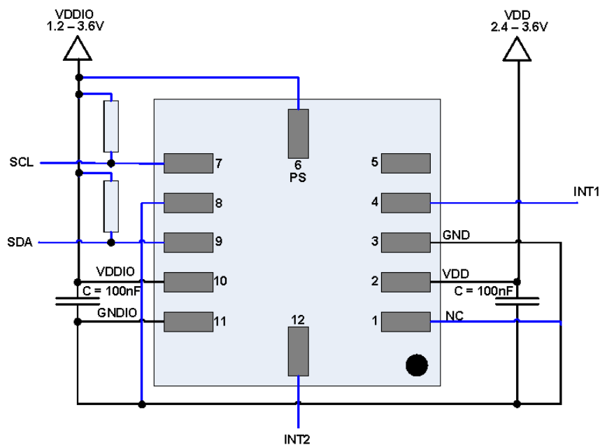
Figure 21: I 2 C connection
